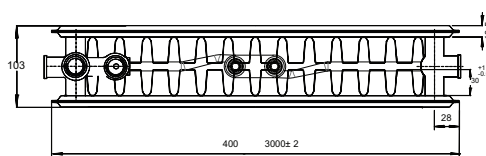
LEFT BOTTOM VIEW
