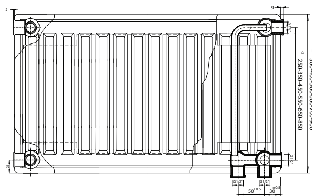
RIGHT VIEW
