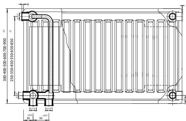
LEFT VIEW
