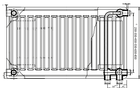
RIGHT VIEW
