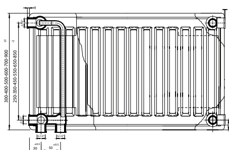
LEFT VIEW
