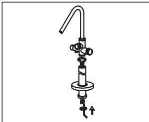
6.Connect body by H8 screw tool,install the decorative cover from top of the pipe,teighten up inlet pipe to the body with H8 hex key.
