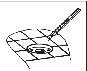
5.Cutting the embeded box along the tiles surface by knife .
