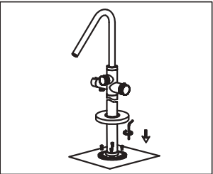
9.Fix pipe in N-box,adjust position, fix plate by M5 screw.
