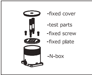
1.N-BOX BOM DRWAING.
