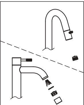
5. After installing faucet, remove the aerator, turn on faucet handle for 1 minute to flush debris. Close the handle and re-assemble the shower.
