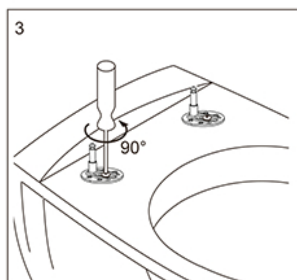
Untighten the screws a bit by turning them 90° in an anti-clockwise direction this will allow you to align the seat.
