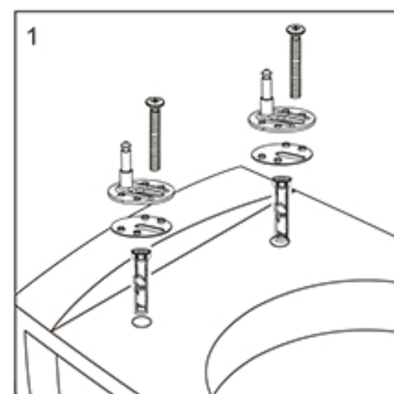
Insert the hinges into the toilet.
